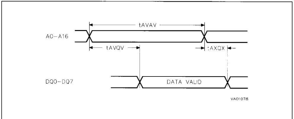
Figure 5. Address Controlled, Read Mode AC Waveforms
