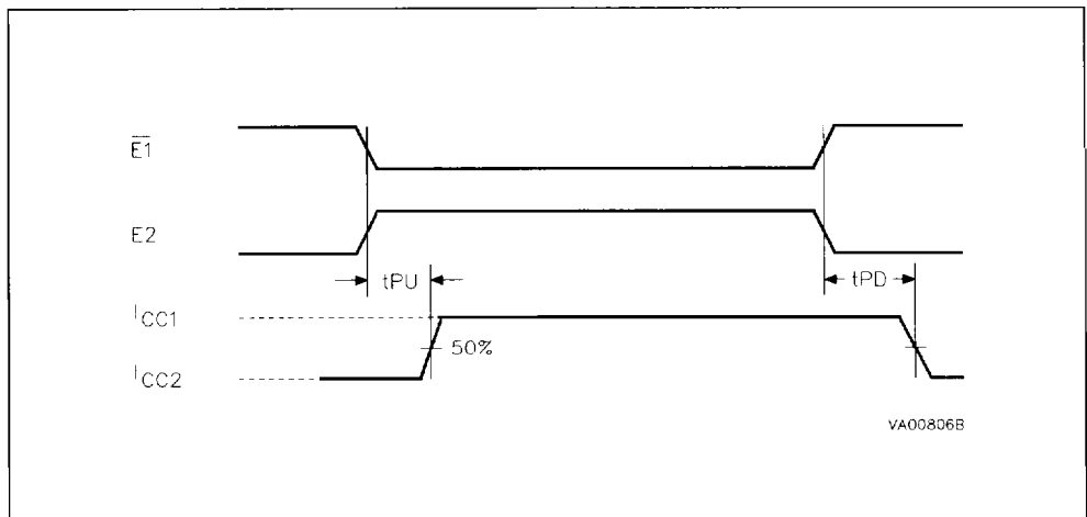
Figure 7. Standby Mode AC Waveforms
